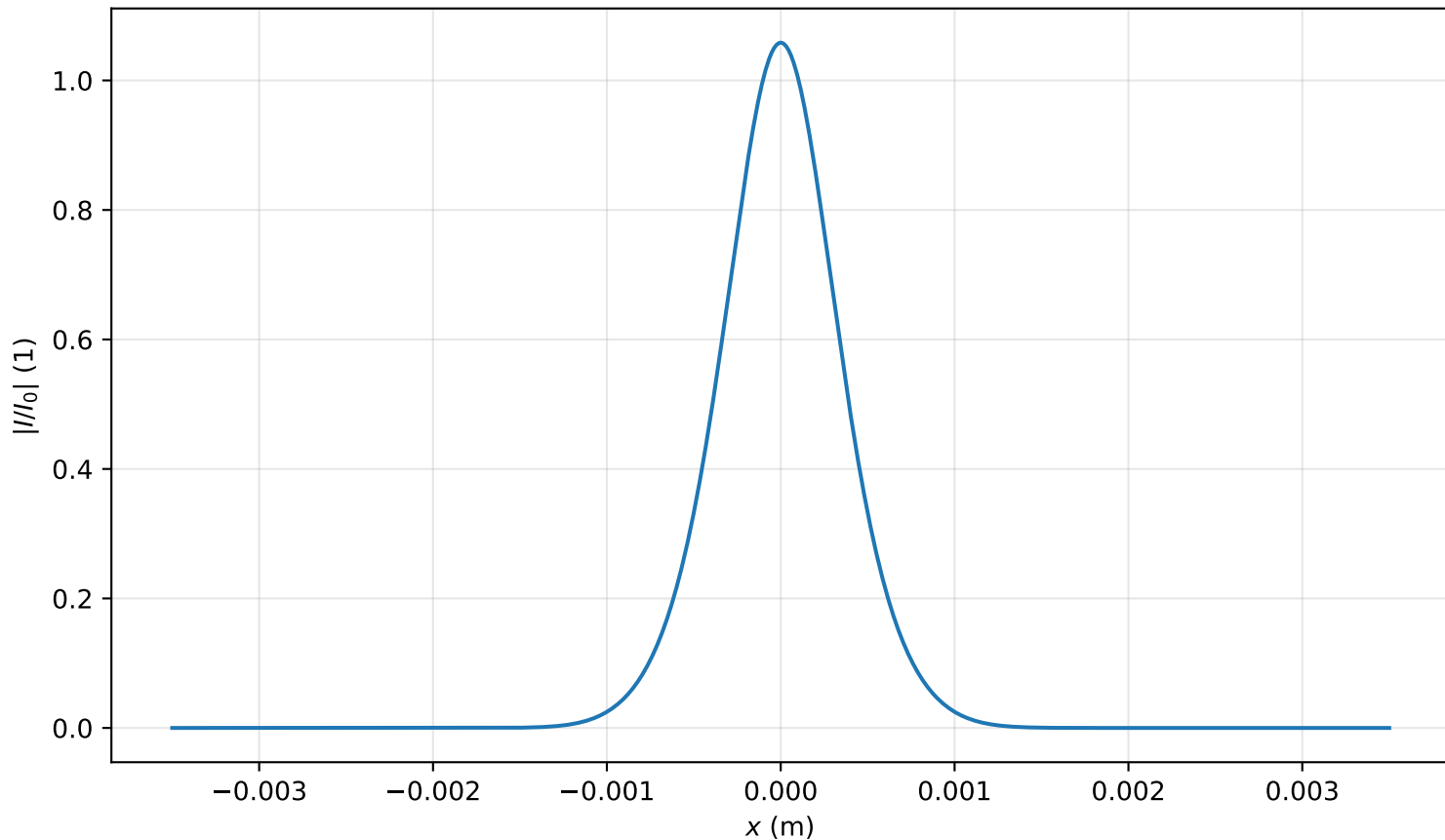
Intensity profile I(x, y = 0, z = 0.876m)/I_0 , P_{in}=0.5P_{cr} , artificial time
